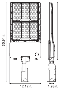
250W / 300W (Slipfitter Mount)
