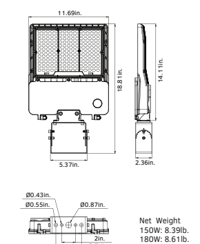
150W / 180W (Yoke Mount)
