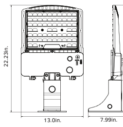
100W/140W/180W (Wall Mount)
