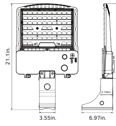
100W/140W/180W (Pole Mount)
