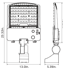
100W/140W/180W (Adjustable Pole Mount)
