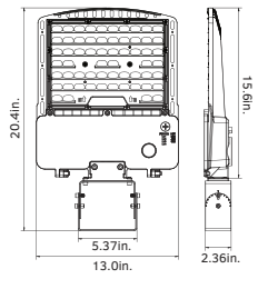
100W/140W/180W (Yoke Mount)
