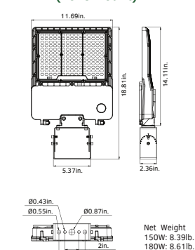
150W / 180W (Yoke Mount)
