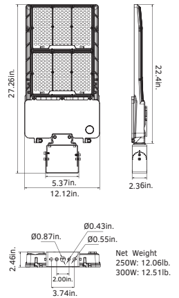
250W / 300W (Yoke Mount)
