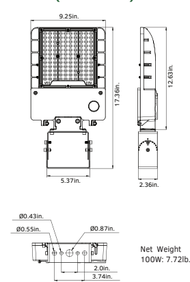
100W (Yoke Mount)
