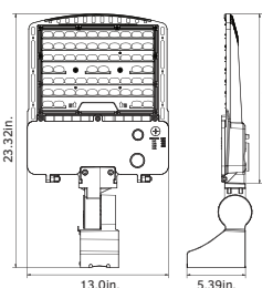
100W/140W/180W (Adjustable Pole Mount)
