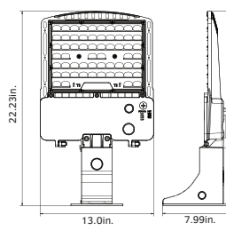
100W/140W/180W (Wall Mount)
