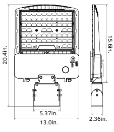
100W/140W/180W (Yoke Mount)
