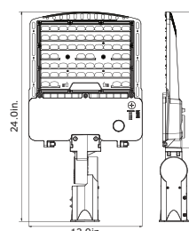
100W/140W/180W (Slipfitter Mount)
