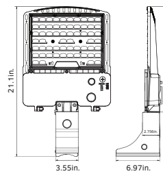
100W/140W/180W (Pole Mount)
